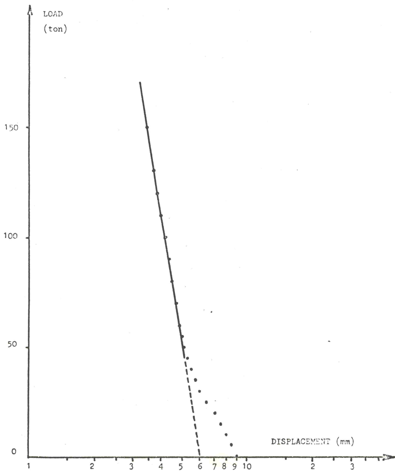
Figure 7 . Piston displacement curve
